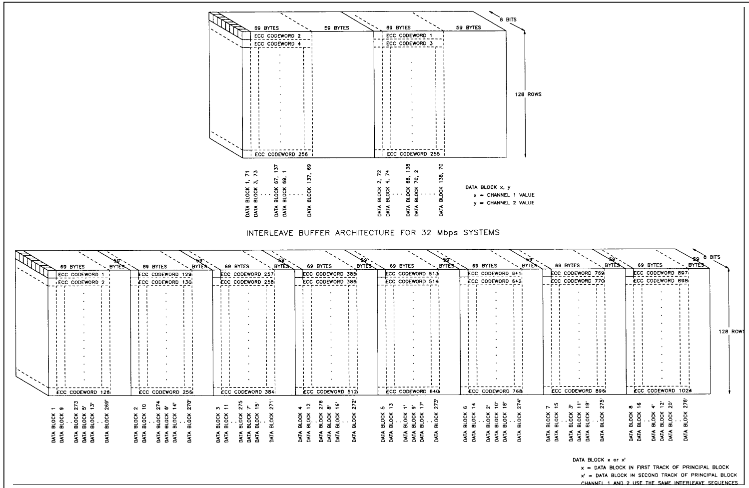
Figure 6-16. Interleave buffer architectures.
