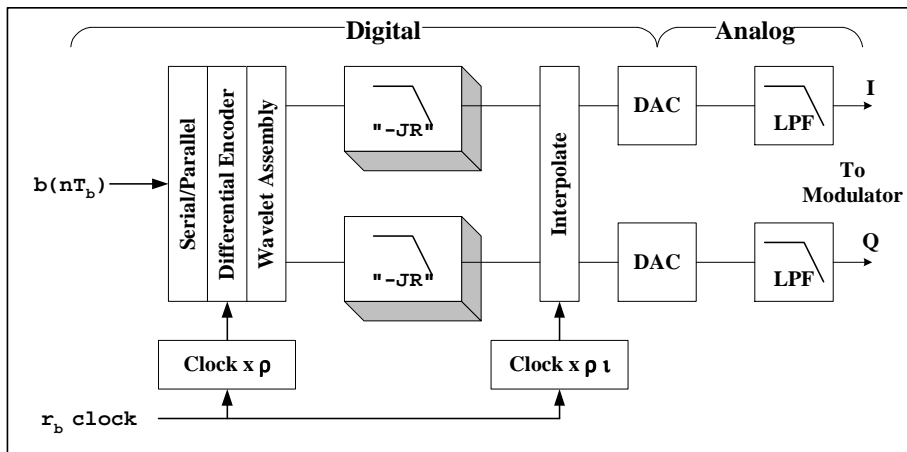
Figure 2-1. FQPSK-JR Baseband Signal Generator
