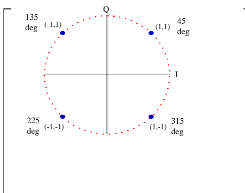
Figure A-15. I & Q constellation.
