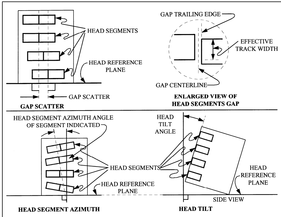
Figure 6-3. Head and head segment mechanical parameters.
