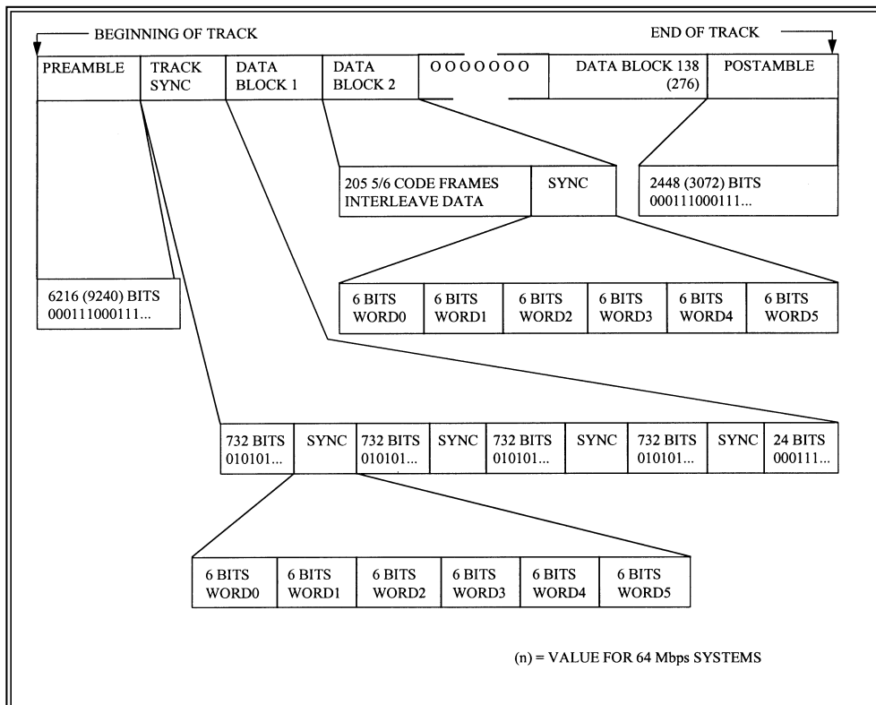
Figure 6-14. Helical track format.
