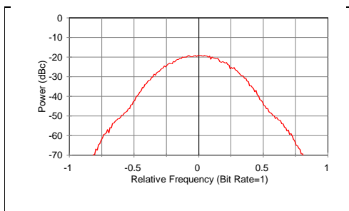
Figure A-23. SOQPSK-TG Power Spectrum (5 Mb/s).
