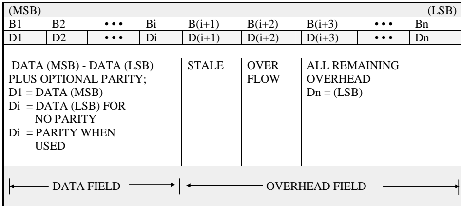
Figure 4-5. Asynchronous word structure.
