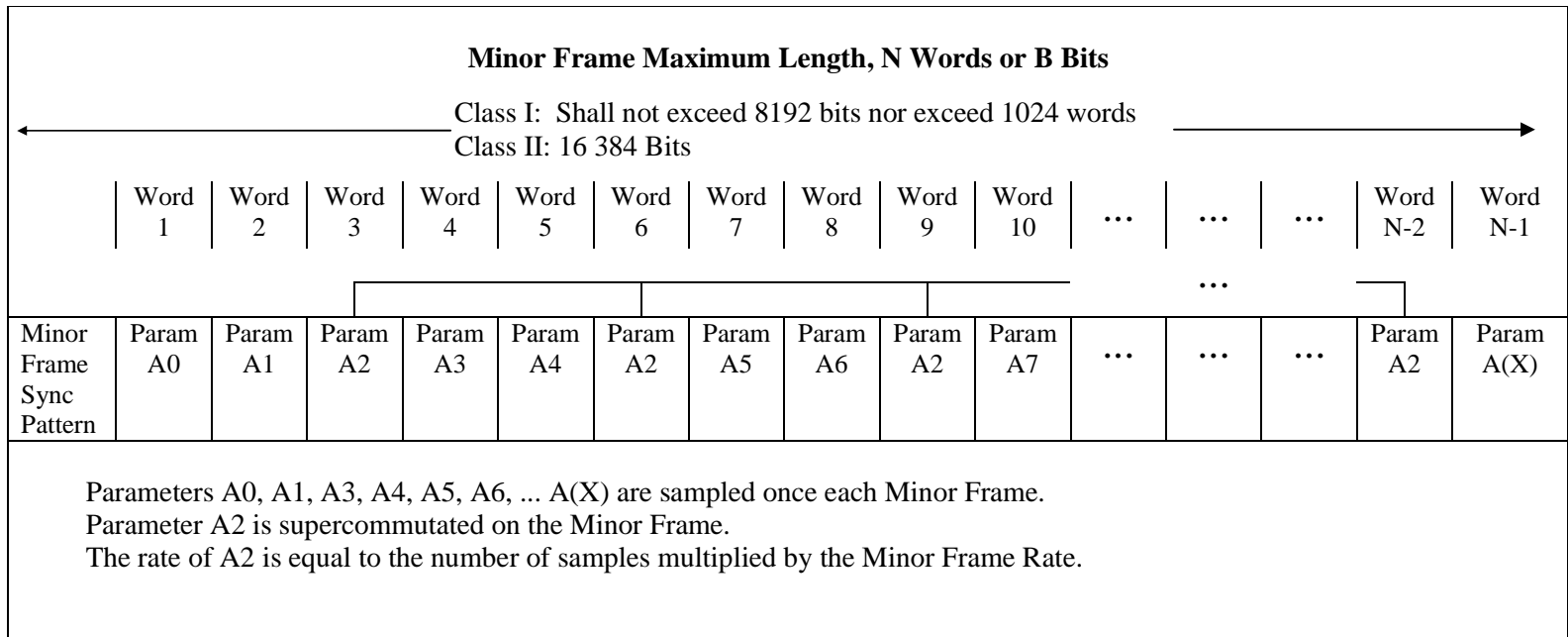
Figure C-4. Major Frame Length = Minor Frame Maximum Length.
