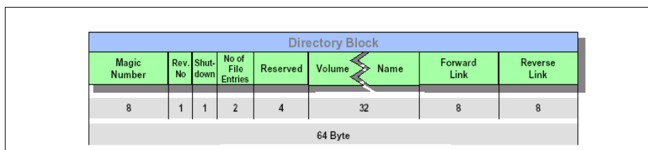
Figure 10-3. Directory Block (as depicted in STANAG 4575).
