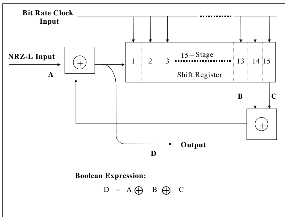
Figure D-2. Randomizer block diagram.
