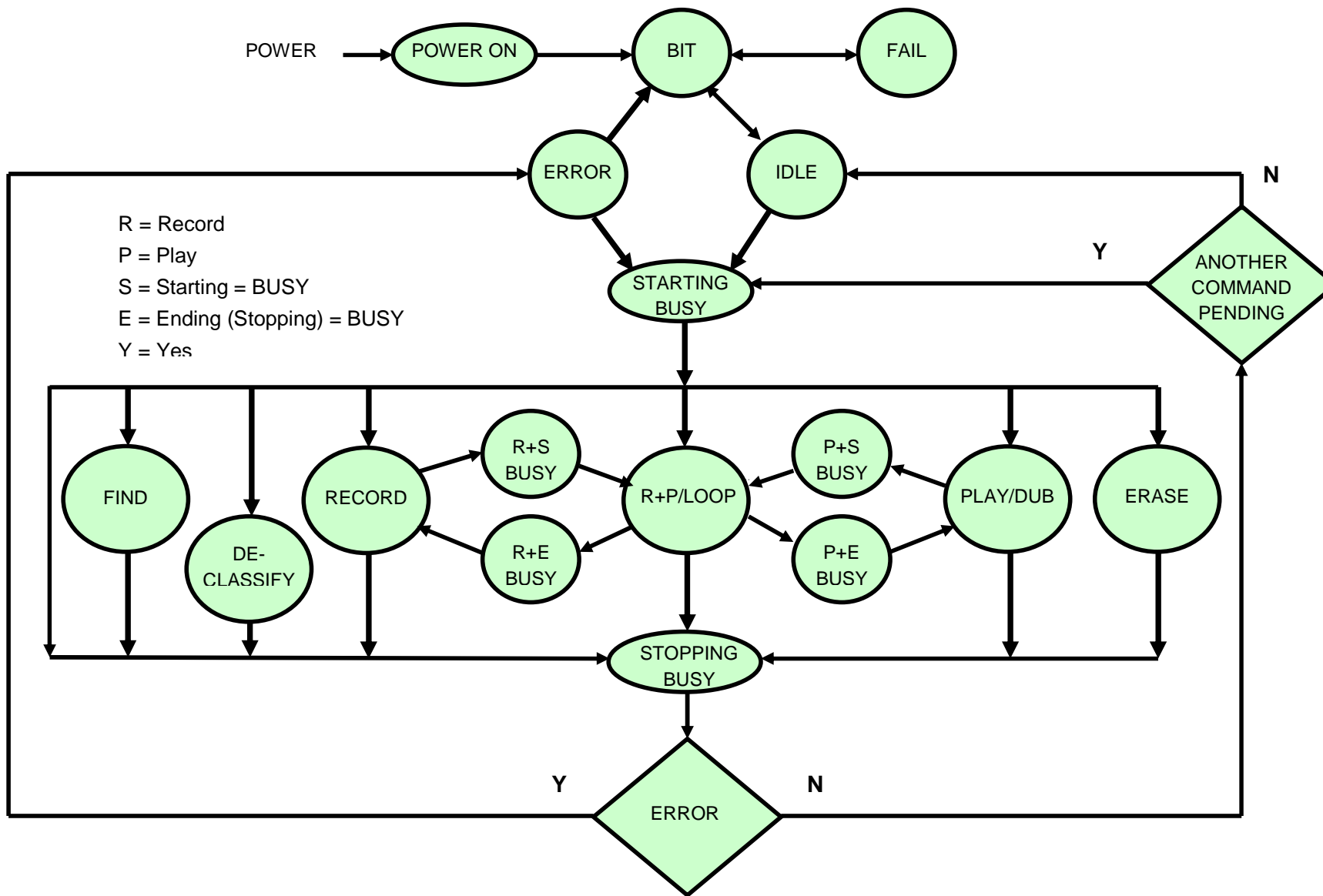
Figure 6-18. Recorder state transition diagram.
