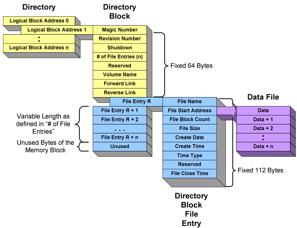
Figure 10-2. Directory Block Structure.
