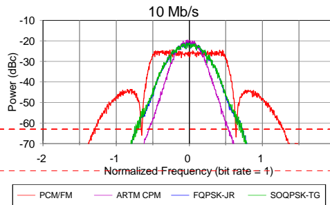
Figure A-1. Spectra of 10-Mb/s CPFSK, ARTM CPM, FQPSK-JR, SOQPSK-TG signals.
