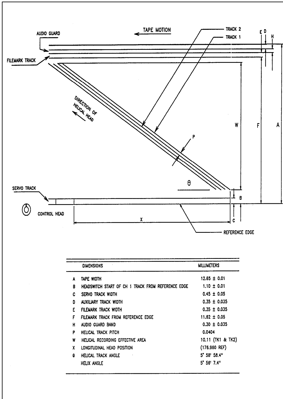
Figure 6-12. Recorded tracks on tape, B format.
