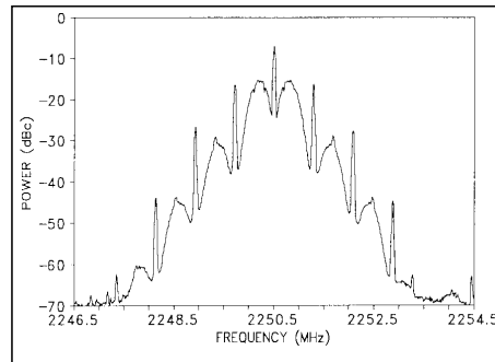
Figure A-6. Biφ PCM/PM signal
