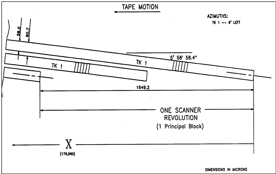
Figure 6-11. Helical track dimensions, E format.
