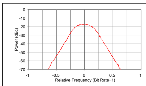
Figure A-25. Power spectrum of 5 Mb/s ARTM CPM.
