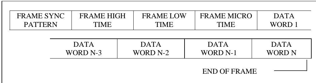
Figure 8-3. Composite frame structure.
