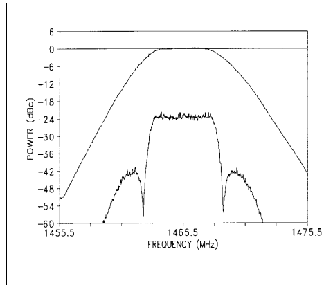
Figure A-5. Spectrum analyzer calibration of 0-dBc level
