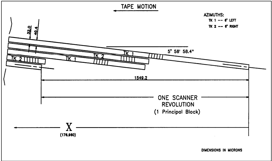
Figure 6-10. Helical track dimensions, B format.
