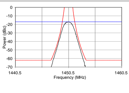
Figure A-13. Typical 5-Mb/s ARTM CPM signal and spectral mask.
