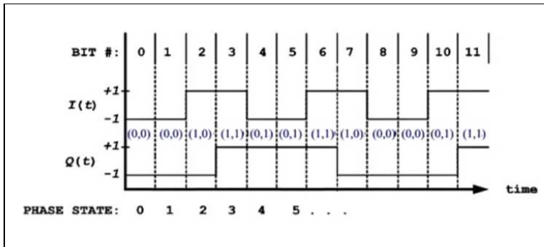
Figure M-5. OFFSET QPSK State Timing.
