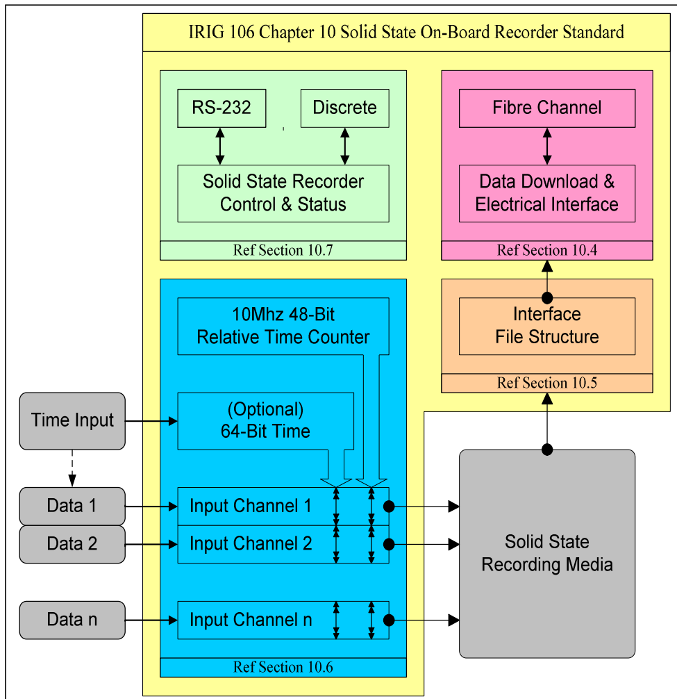
Figure 10-1. Functional layout of standard.
