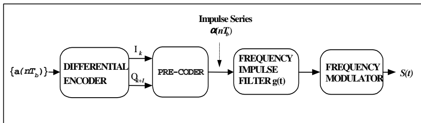
Figure 2-3. SOQPSK Transmitter.
