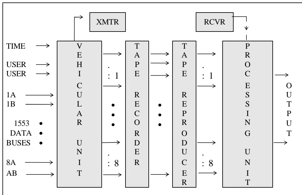
Figure 8-1. System block diagram.
