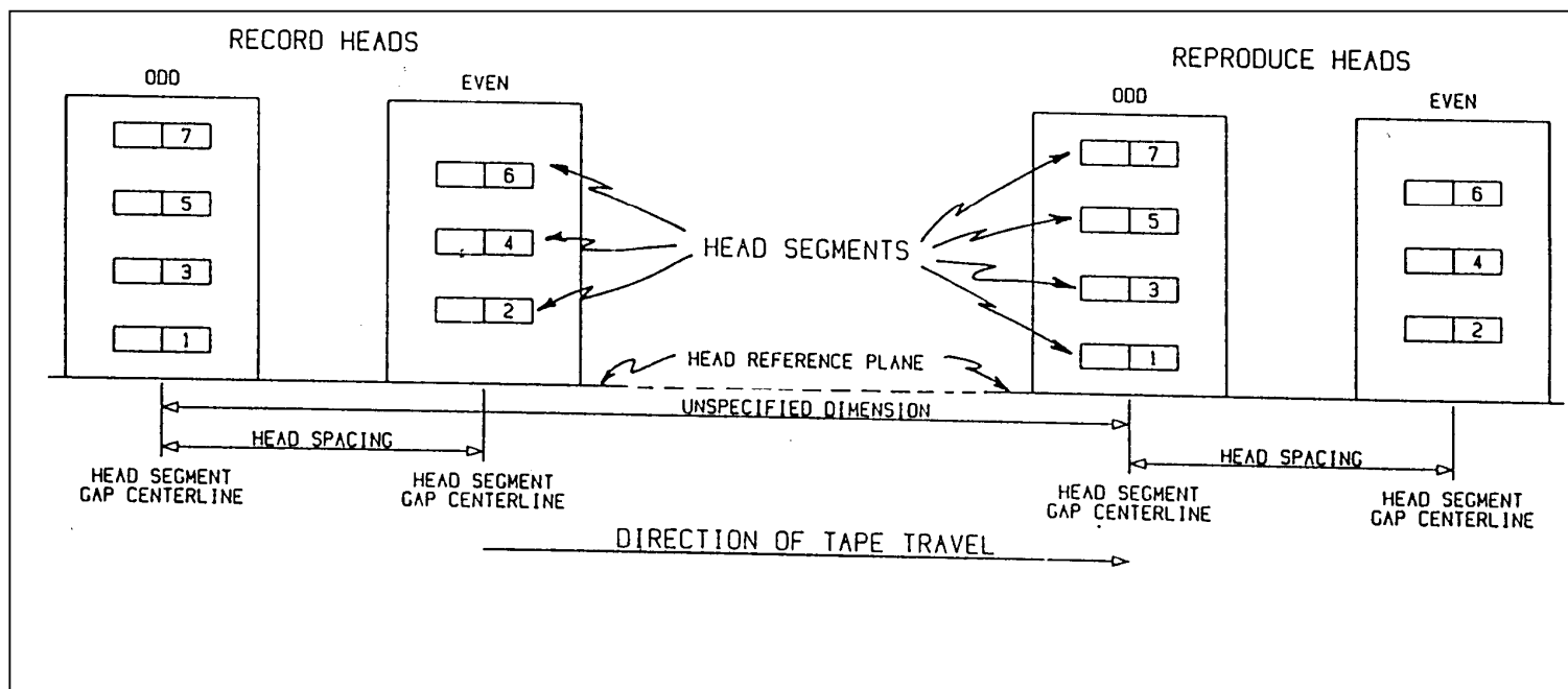
Figure D-1. Record and reproduce head and head segment identification and location (7-track interlaced system).
