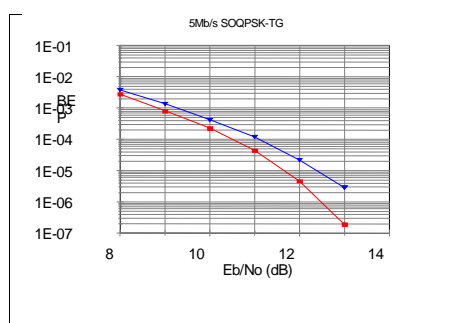
Figure A-24. BEP versus E_b/N_0 performance of 5 Mb/s SOQPSK-TG.
