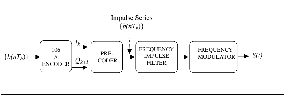
Figure M-7. OQPSK Transmitter (with precoder).
