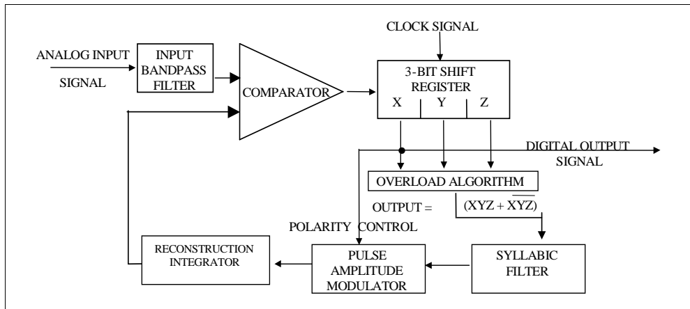
Figure F-1a. Typical CVSD encoder.
