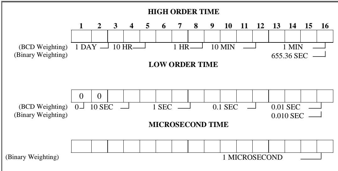
Figure 4-3 16 bit standardized time word format.
