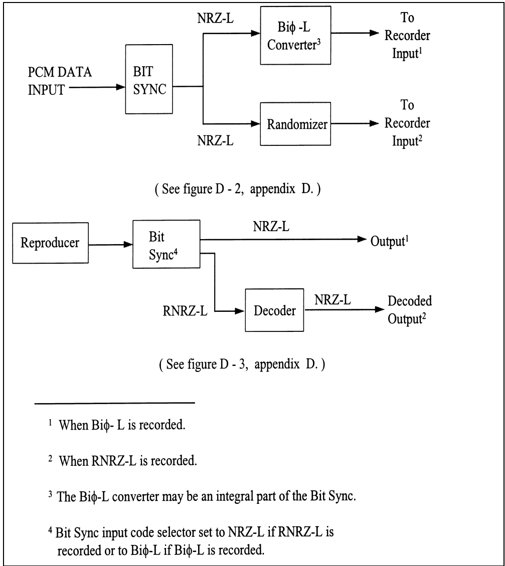
Figure 6-5. Serial high-density digital record and reproduce.
