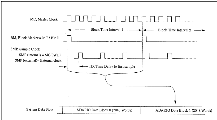
Figure G-3. ADARIO timing.
