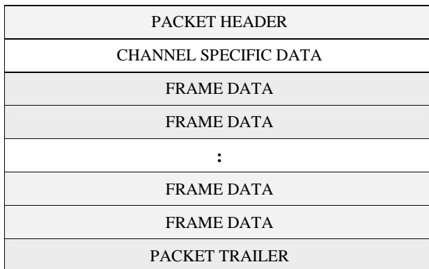
Figure 10-43. General MPEG-2 Video Packet, Format 0.
