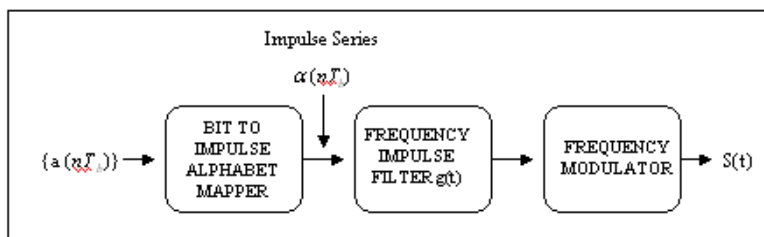
Figure 2-2. Basic SOQPSK.
