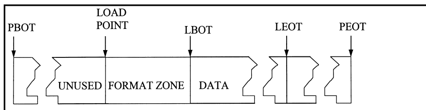
Figure 6-13. Tape cartridge layout.
