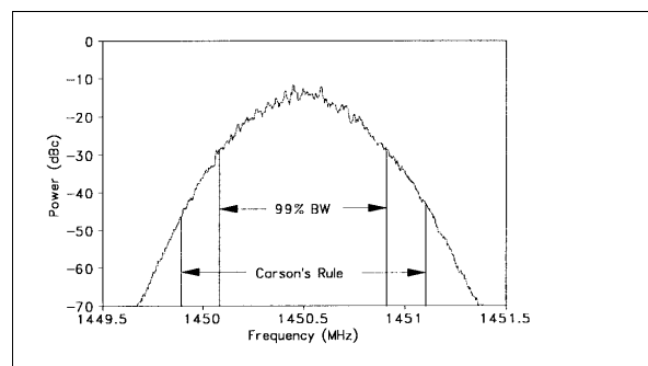
Figure A-7. FM/AM signal and Carson's Rule
