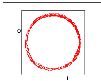
Figure A-18. FQPSK-B vector diagram.
