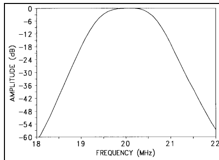
Figure A-8. Typical receiver RLC IF filter response (-3 dB bandwidth = 1 MHz).
