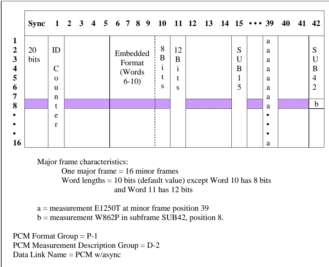
Figure J-2. PCM format for PCM w/async.
