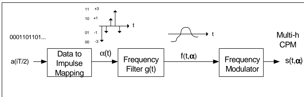
Figure 2-4. Conceptual CPM modulator.
