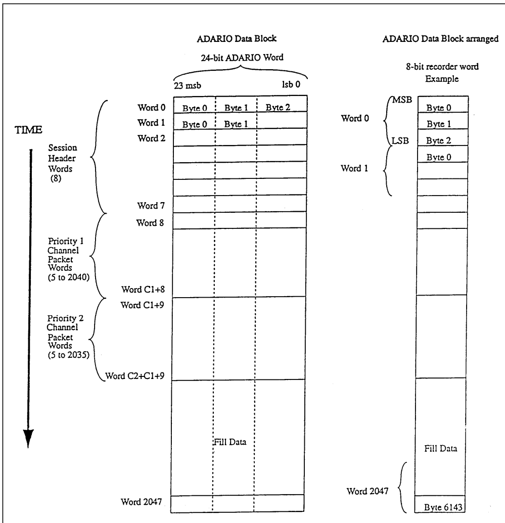
Figure G-2. ADARIO data blocks.
