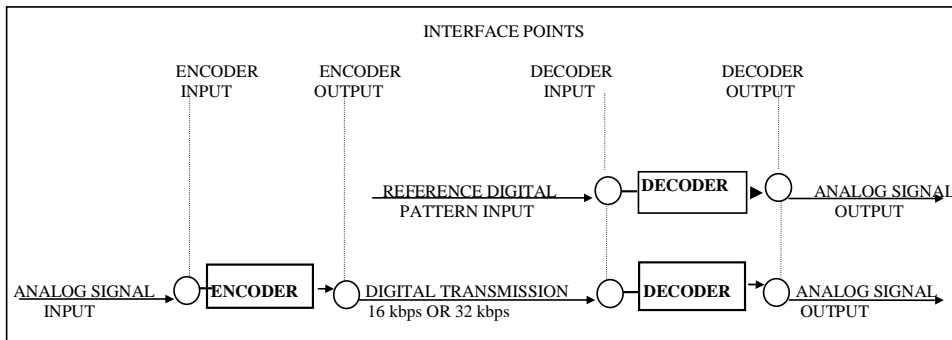
Figure F-3. Interface diagram for CVSD converter.
