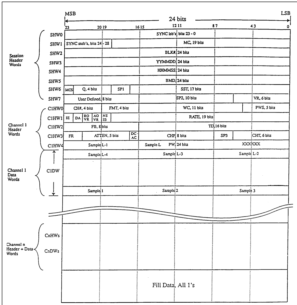
Figure G-1. ADARIO data format.
