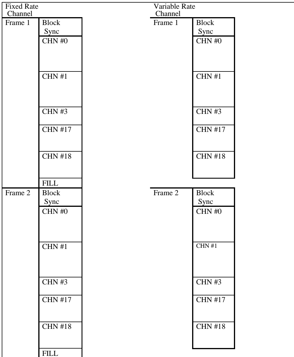
Figure G-5. Submux aggregate format.
