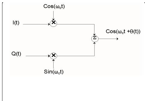
Figure A-14. OQPSK modulator.
