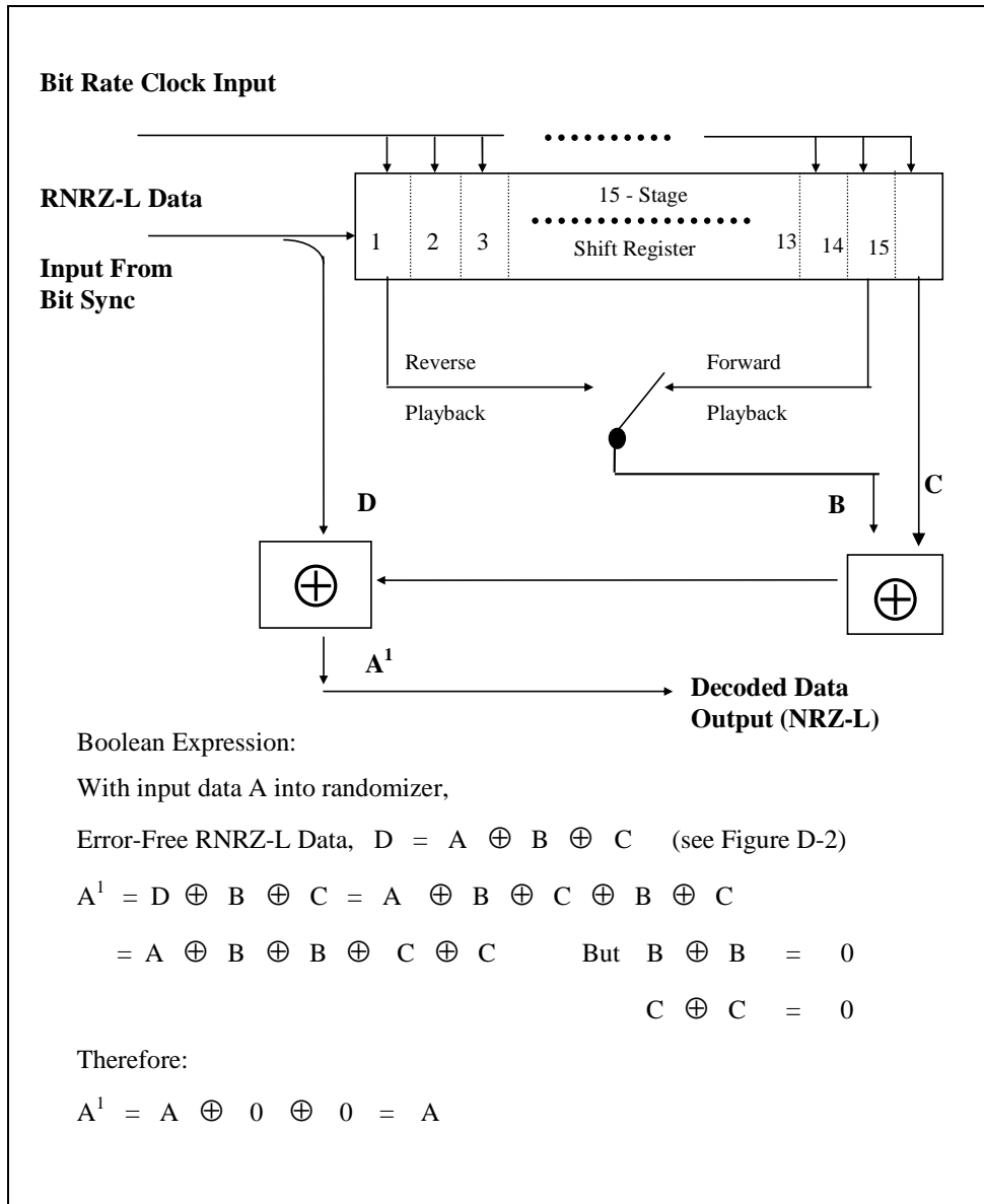
Figure D-3. Randomized NRZ-L decoder block diagram.
