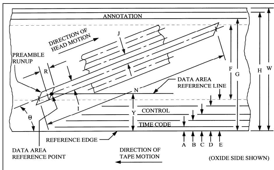
Figure 6-6. Location and dimensions of recorded tracks.
