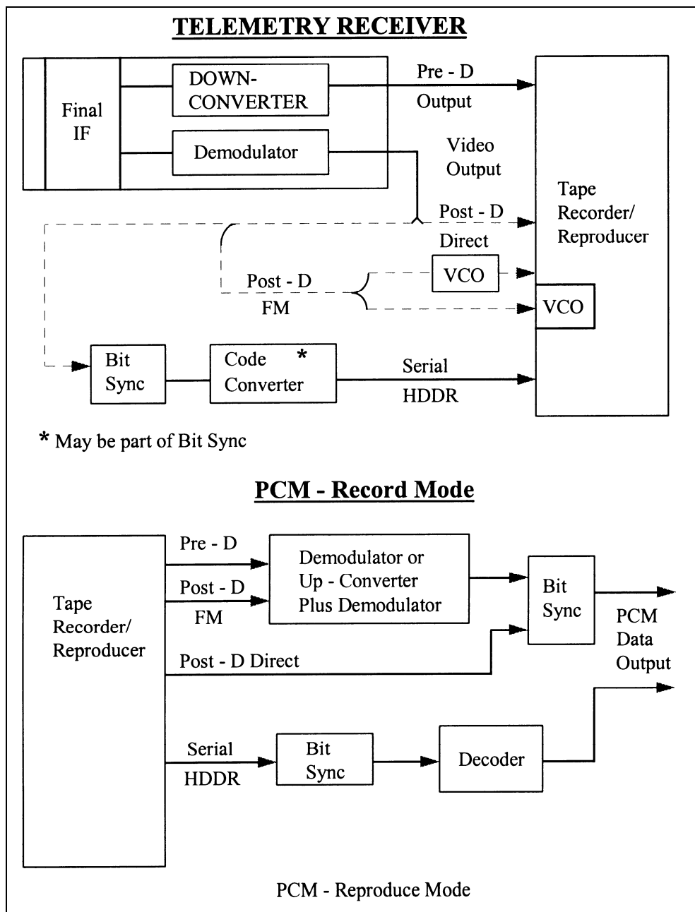
Figure 6-4. PCM record and reproduce configuration.
