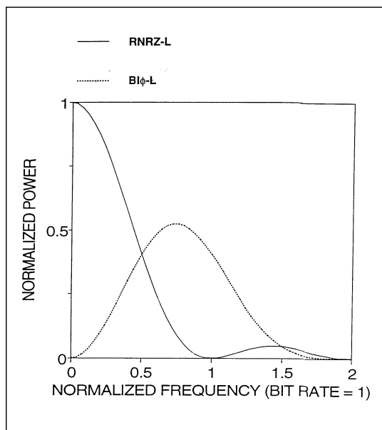
Figure D-4. Random PCM power spectra.
