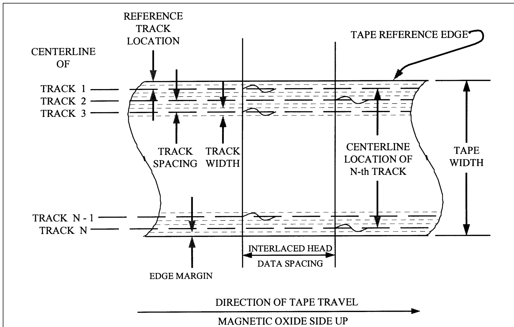
Figure 6-1. Recorded tape format.
