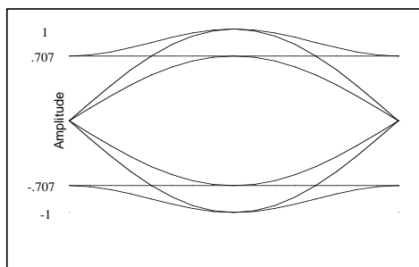
Figure A-16. FQPSK wavelet eye diagram.
