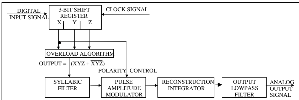
Figure F-1b. Typical CVSD decoder.
