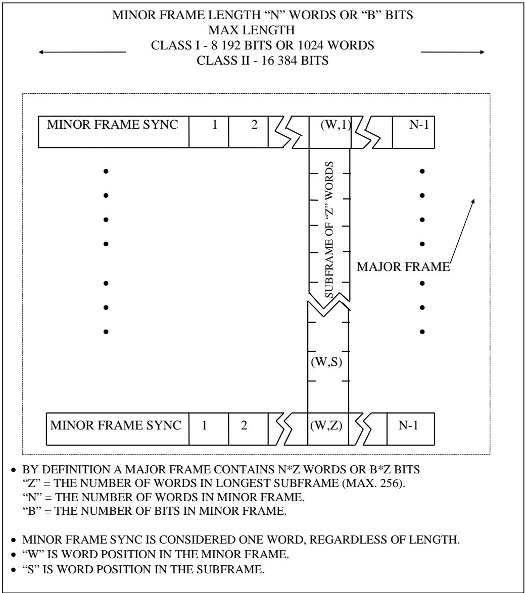
Figure 4-2. PCM frame structure.
