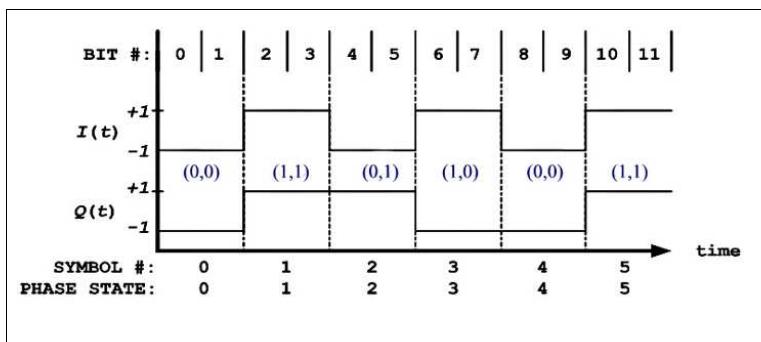
Figure M-4. QPSK State Timing
