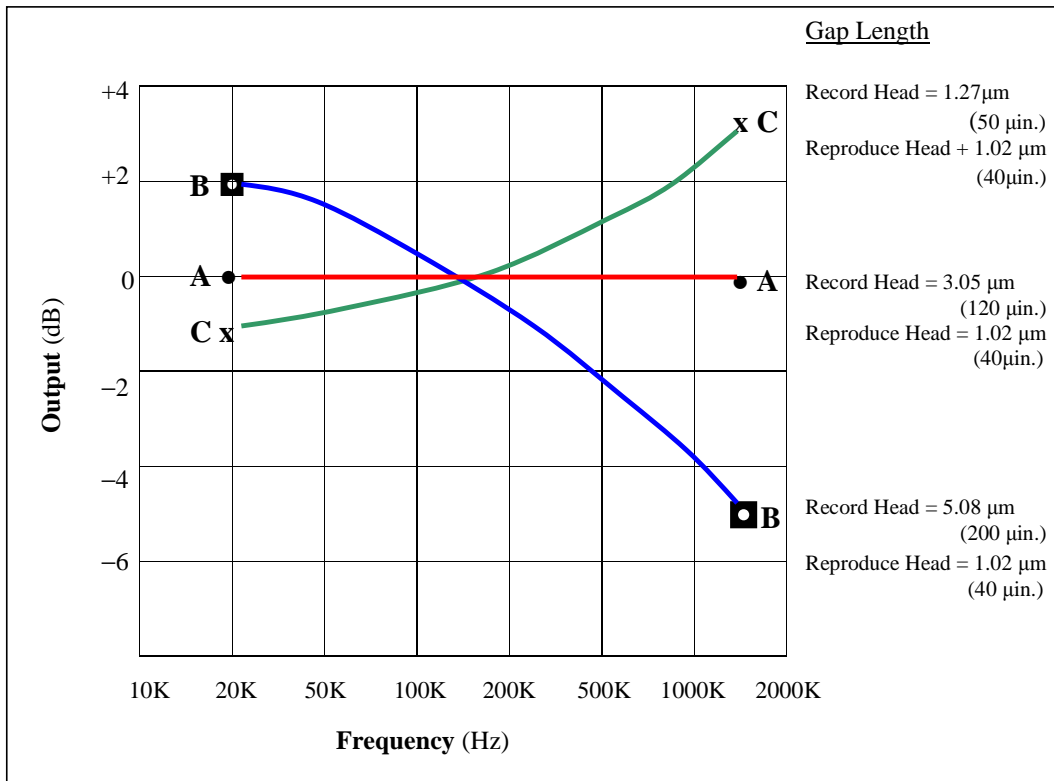
Figure D-6. Tape crossplay.
