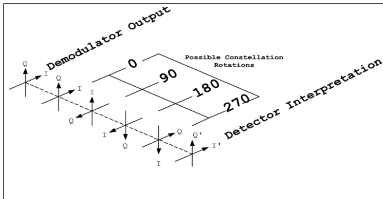
Figure M-3. Detection ambiguity.
