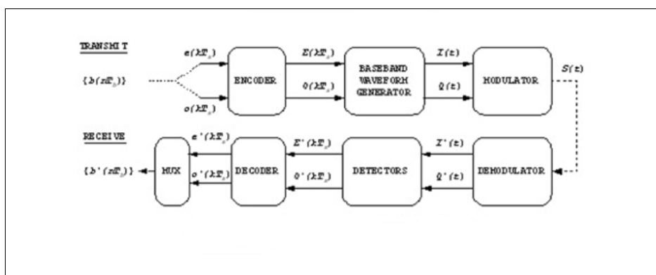
Figure M-1. Transmission System.
