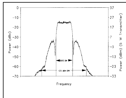
Figure A-4. RNRZ PCM/FM signal.
