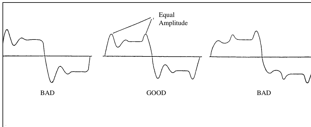
Figure D-7. Square wave responses.
