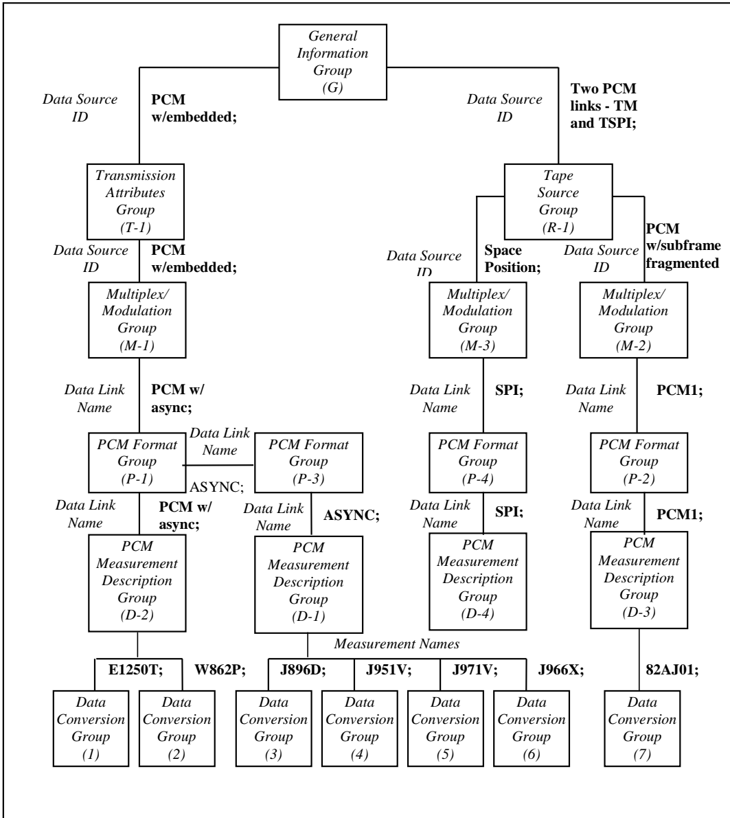
Figure J-1. Group linkages.
