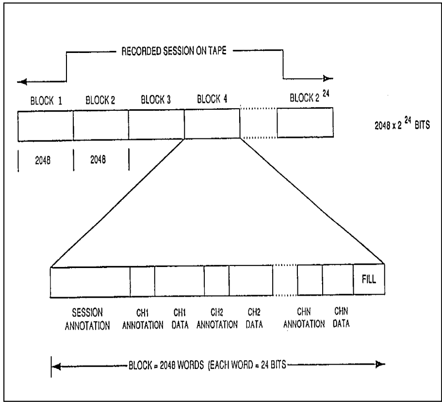
Figure 6-7. ADARIO block format.
