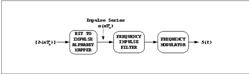
Figure M-6. Basic SOQPSK Transmitter.
