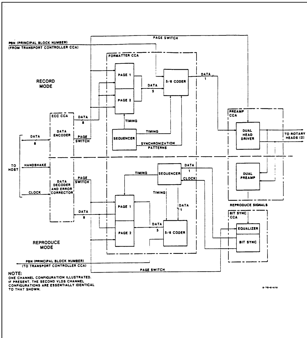
Figure 6-15. Typical VLDS data path electronics block diagram.
