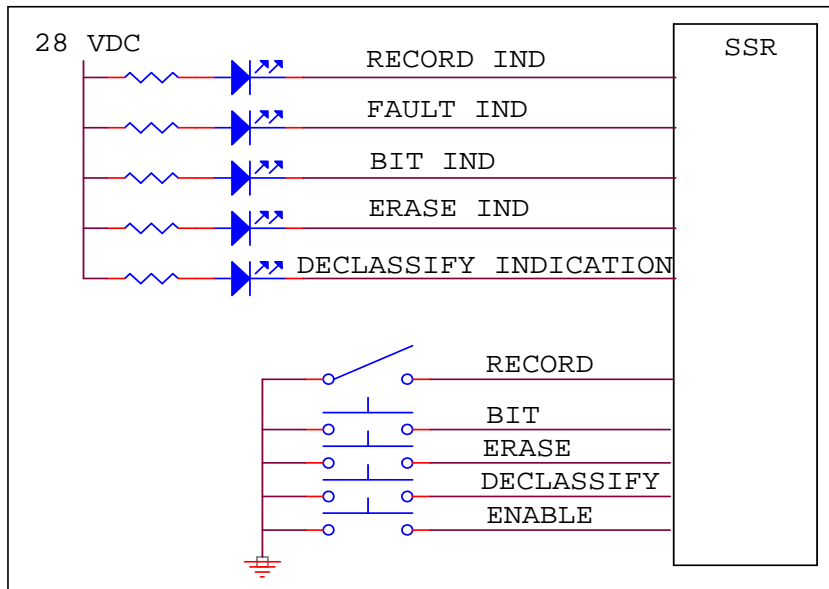
Figure 10-55. Discrete Control and Indicator functional diagram.
