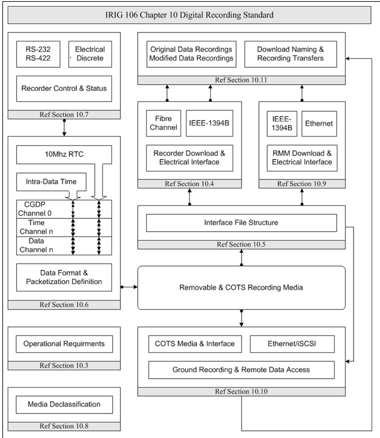
Figure 10-1. Functional Layout of Digital Recorder Standard
