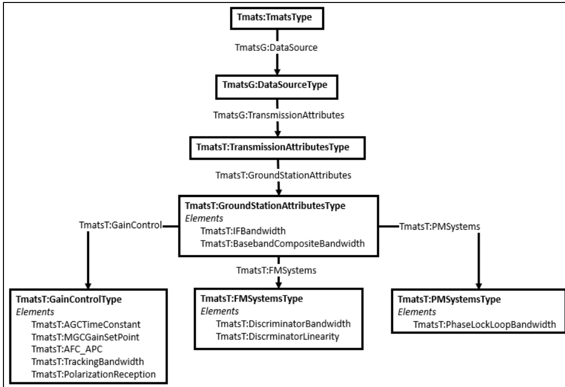
Figure 5-36. Ground Station Attributes Group Example XML Schema
