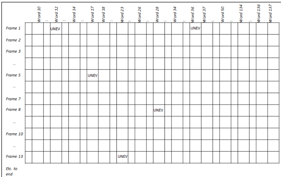
Figure 5-31. Unevenly Spaced Measurements
