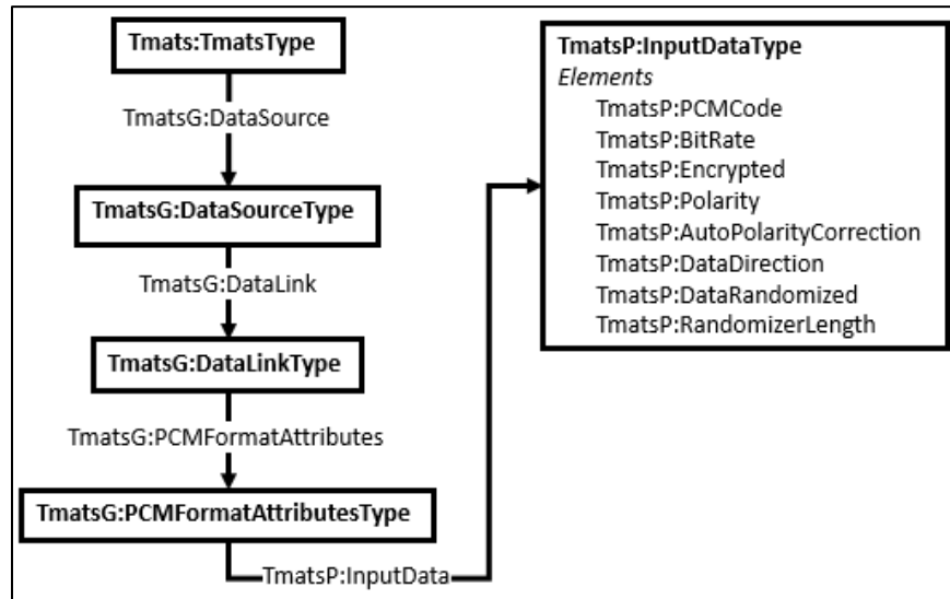
Figure 3-9. PCM Format Attributes Group Example XML Schema
