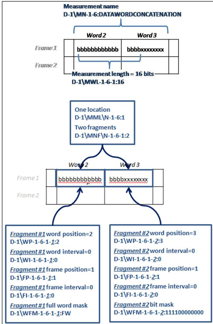
Figure 5-25. Concatenation Example 1: Two Words
