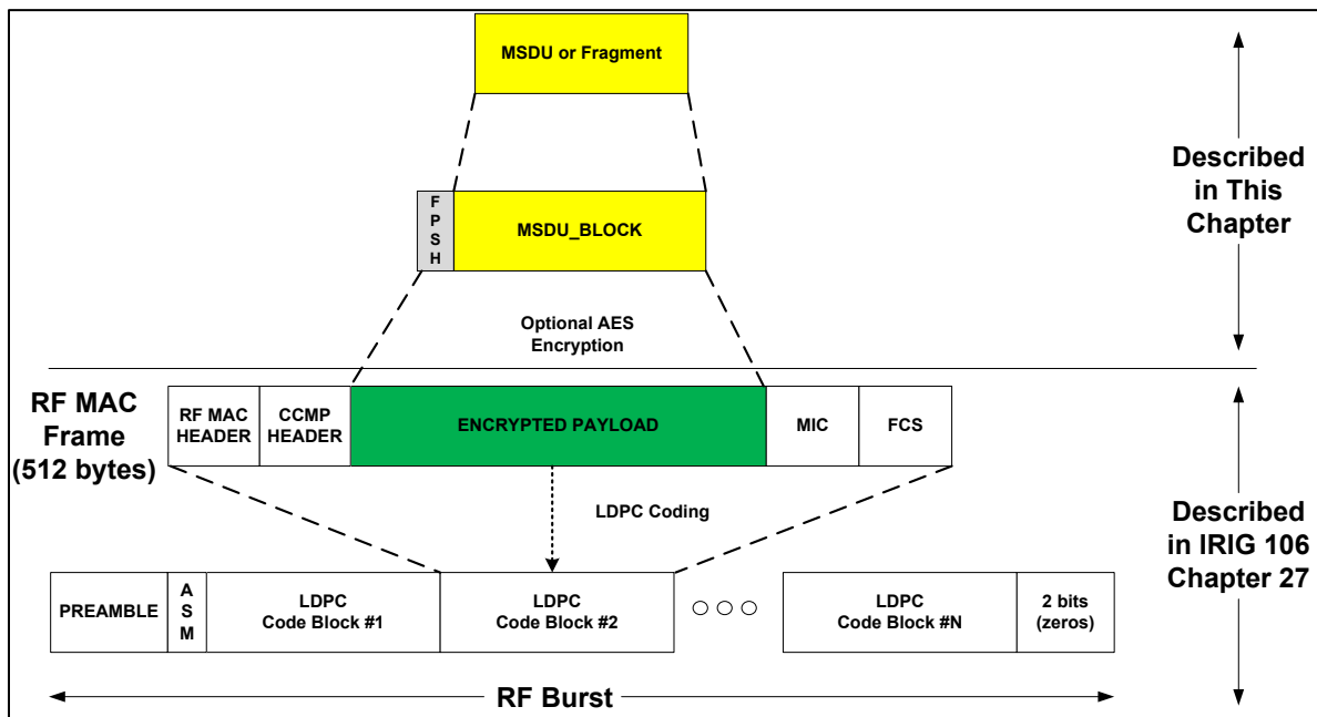
Figure 28-4. MSDU Insertion into RF MAC Frame
