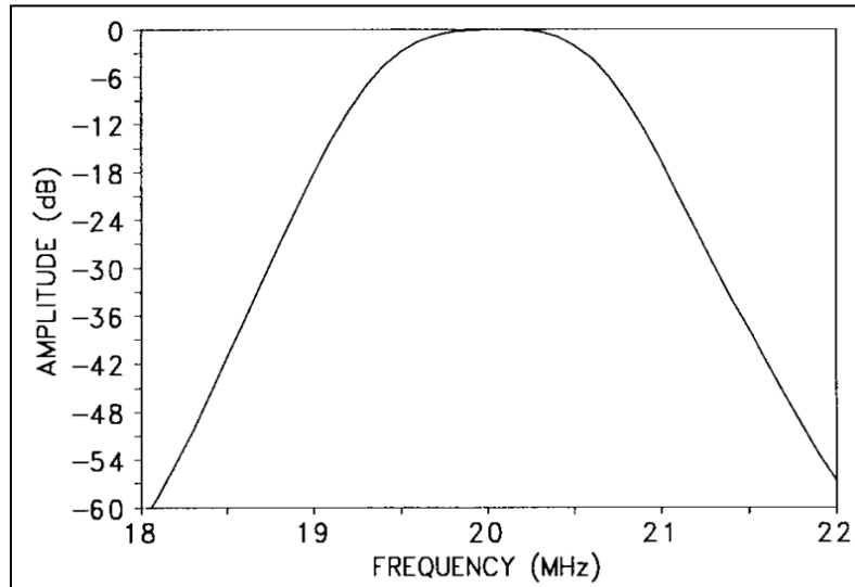
Figure A-15. Typical Receiver RLC IF Filter Response ( -3 dB Bandwidth = 1 MHz)
