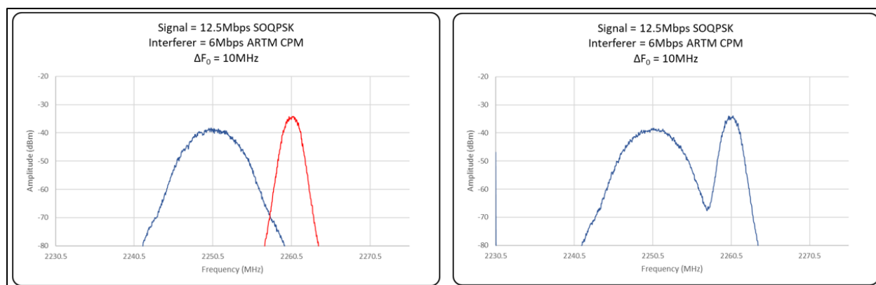
Figure A-3. Center Frequency Spacing 12.5 Mbps PCM/FM and 6 Mbps ARTM CPM
