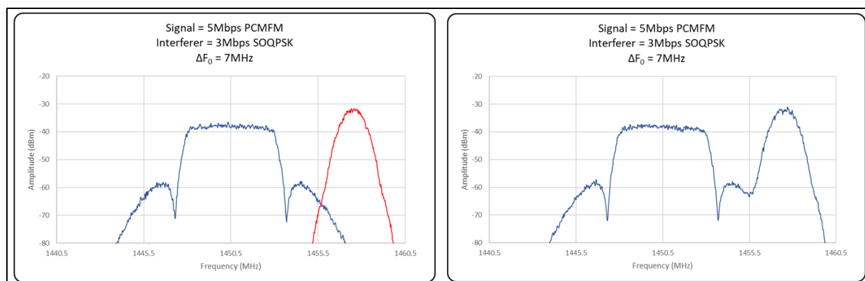
Figure A-2. Center Frequency Spacing 5 Mbps PCM/FM and 3 Mbps SOQPSK-TG
