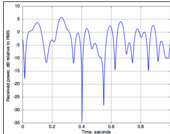
Figure F-9. Rayleigh Fading of a Signal Transmitted from a Moving Platform 68
