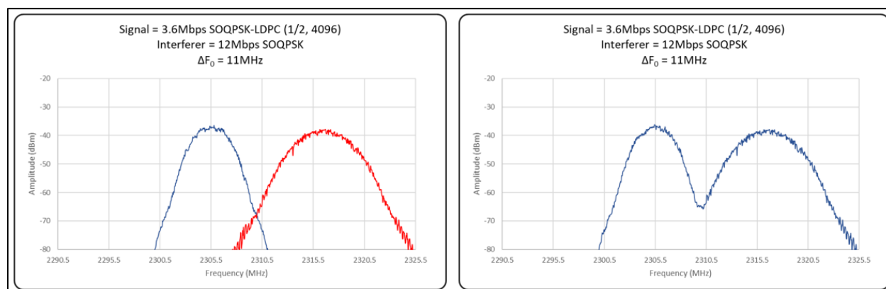
Figure A-6. Center Frequency Spacing 3.6 Mbps SOQPSK-LDPC and 12 Mbps SOQPSK-TG
