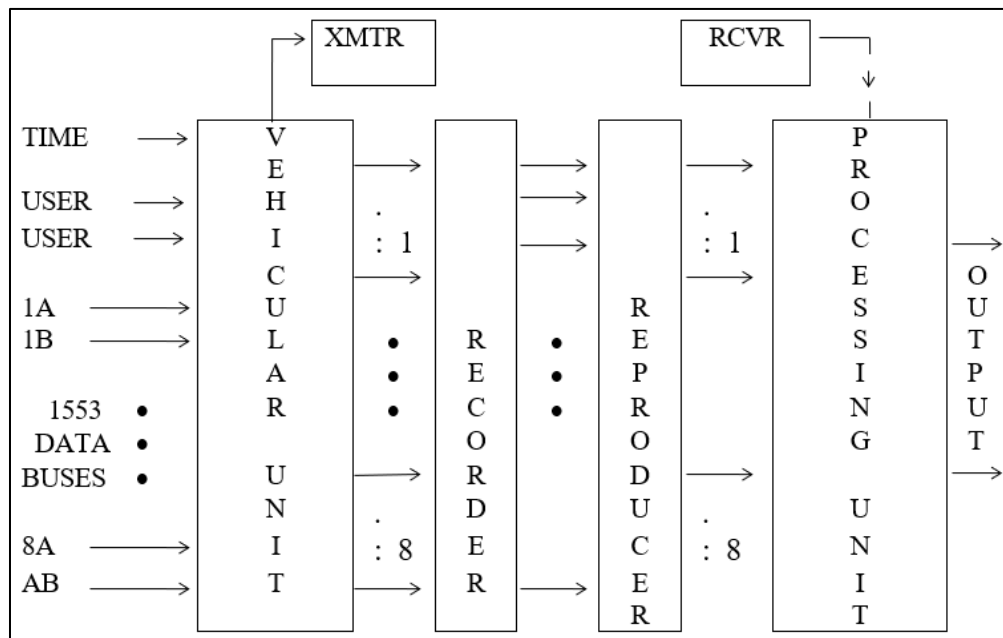
Figure 8-2. System Block Diagram
