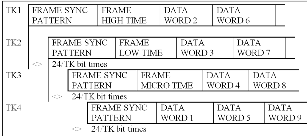
Figure A-1. Multiple Tape Track Spread Format (4-Track Spread Example)
